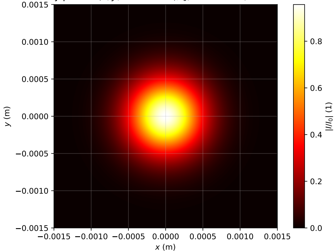
Intensity profile I(x, y, z = 0.876m)/I_0 , Pin=0.3Pcr, artificial time
